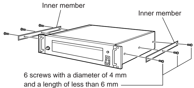
Inner member installation
